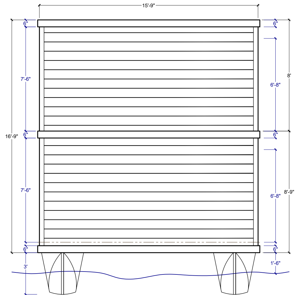
○ BOW ELEVATION
